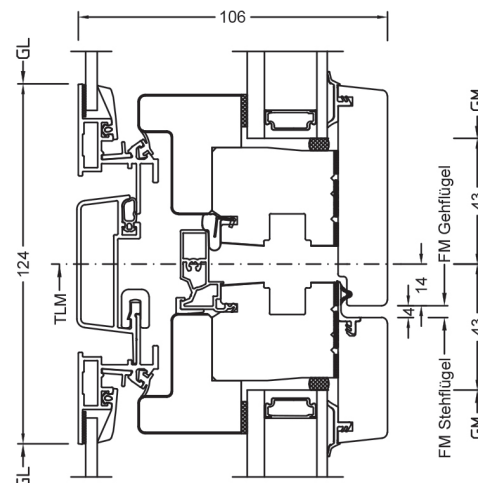
Flying mullion
