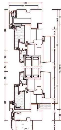
Vertical with installed window
