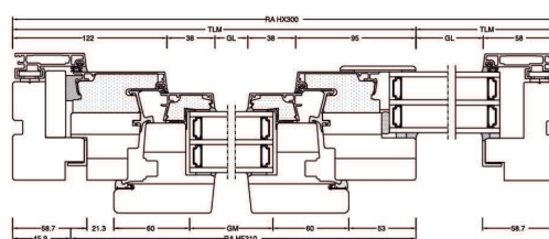
Horizontal with installed window
