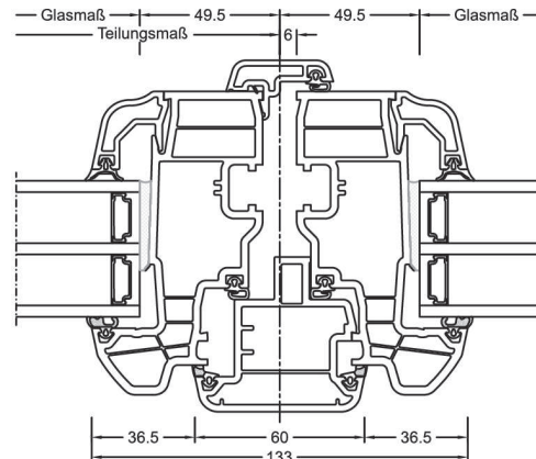
Flying mullion
