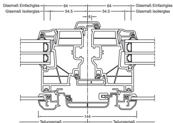
Flying mullion
