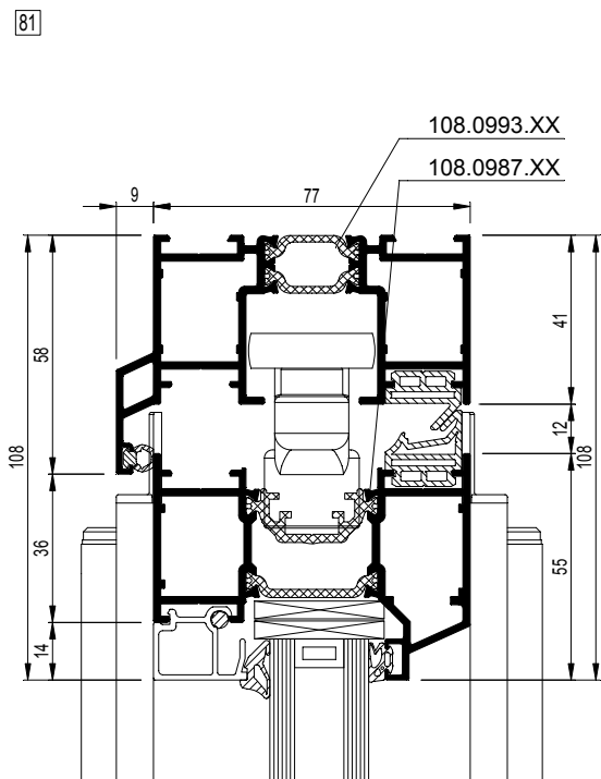
CF77-081001.dxf CF77-081001.dwg
