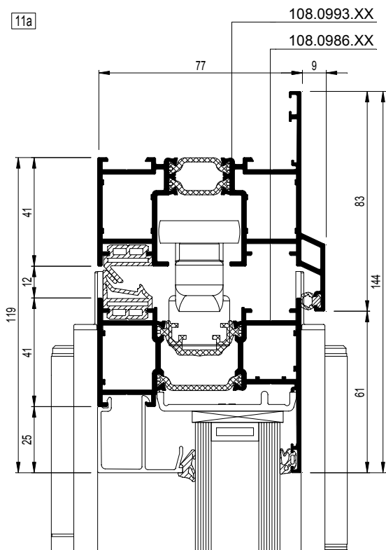
CF77-011002.dxf CF77-011002.dwg
