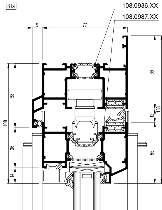
CF77-081002.dxf CF77-081002.dwg
